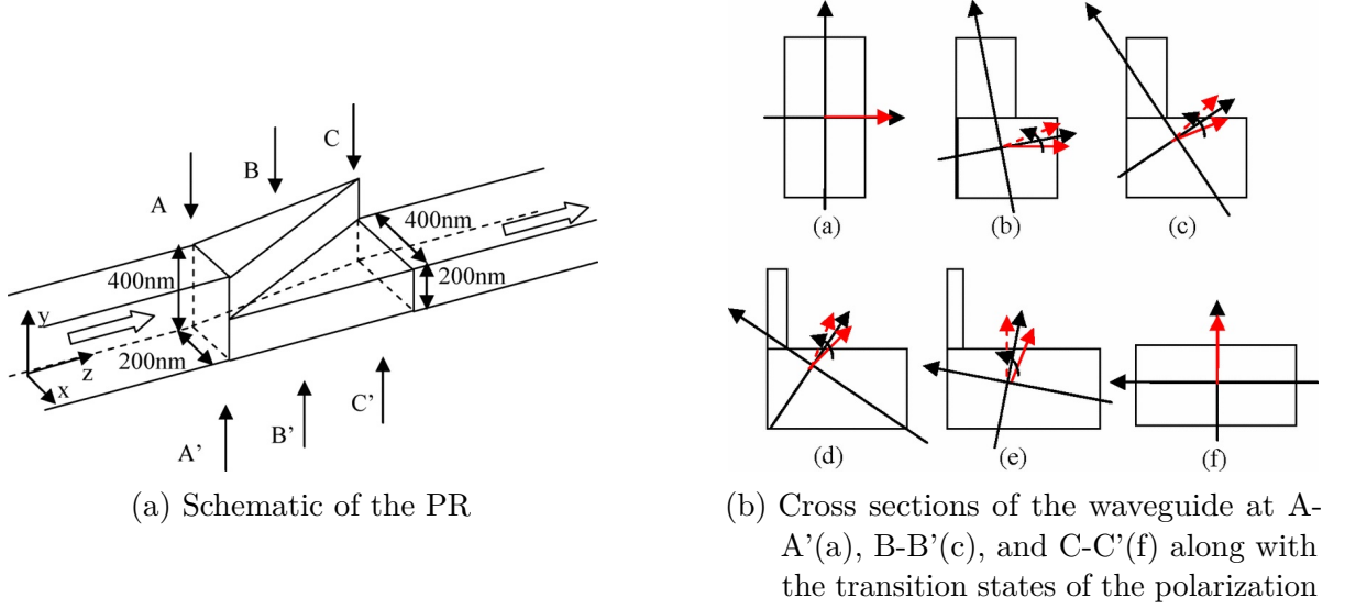
Figure 3.2: PR using mode evolution, by Zhang et al. [51]
