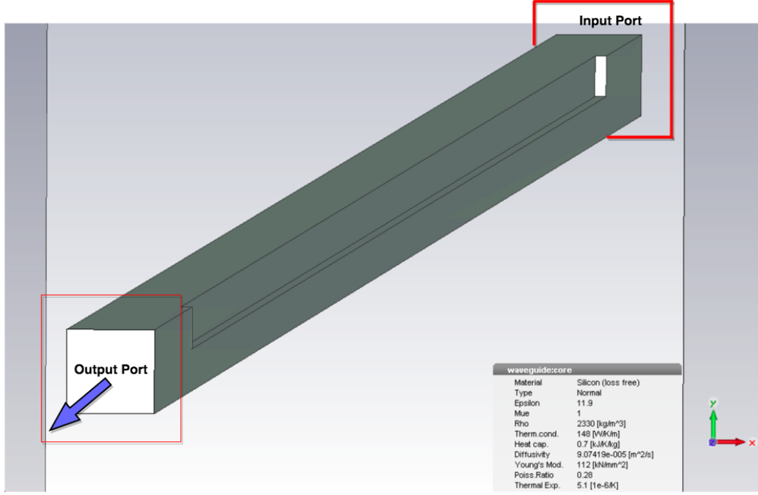
Figure 4.6: Design of single-stair waveguide with initial dimensions at the port as width = 230 nm and height = 220 nm. Stair cross-section dimensions are: Rib width = 200 nm, Rib height = 110 nm, Base width = 230 nm, Slab height = 110 nm, and cross-section length = 62 \mu\text{m} . The output port is along the Z-axis, shown in the figure
