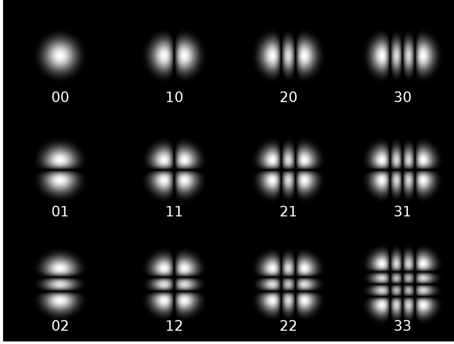
Figure 2.3: TEM modes labelled with corresponding indices. The indices describe the shape of the modes as m+1 columns and n+1 rows. i.e. \text{TEM}_{21} mode shape has 3 columns and 2 rows.
