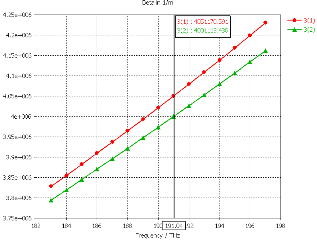
Figure 4.5: Simulated effective propagation constant for the port modes in the cross-section of \text{Rib}_{\text{width}} = 200 \text{ nm} , \text{Rib}_{\text{height}} = 110 \text{ nm} , \text{Base}_{\text{width}} = 230 \text{ nm} , \text{Slab}_{\text{height}} = 110 \text{ nm} , obtained using CST simulation
