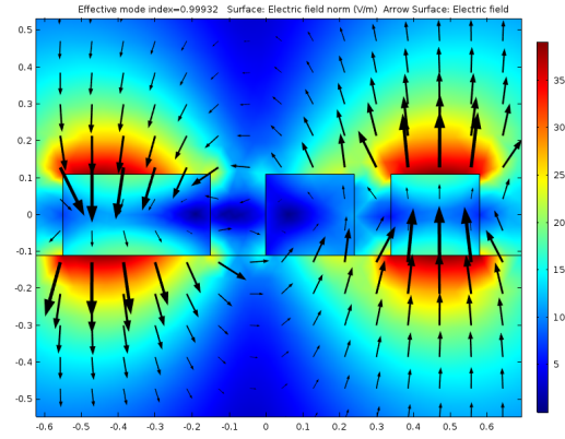
(b) Phase mismatched TM coupling in the mode coupling cross-section
