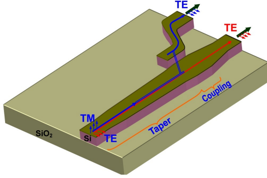
(a) Structure of the PR
