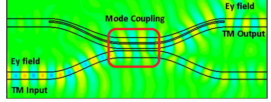
(b) TM mode crossing at the coupling region
