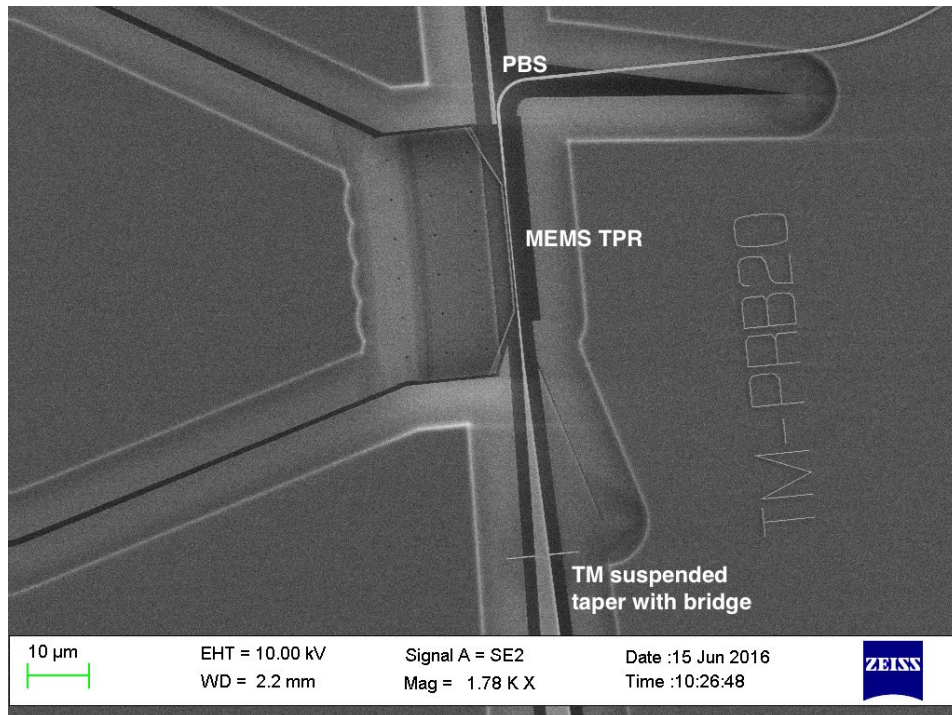
Figure 5.5: TM input with tapers, PBS and MEMS cantilever viewed under SEM
