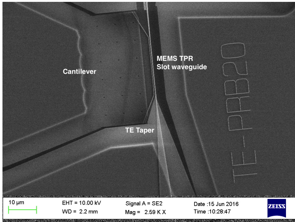
Figure 5.3: TE input with tapers, PBS and MEMS cantilever viewed in SEM
