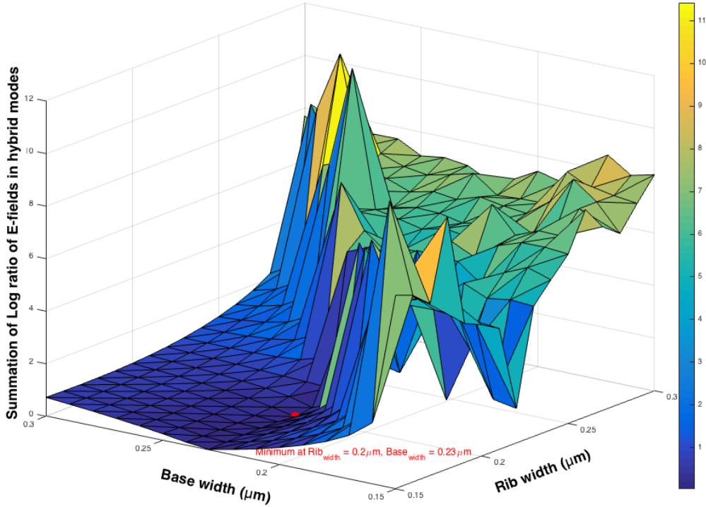
Figure 4.2: Summation of real part of absolute value of the logarithmic ratio of E_x and E_y fields plotted against rib and base width in an area chart using MATLAB
