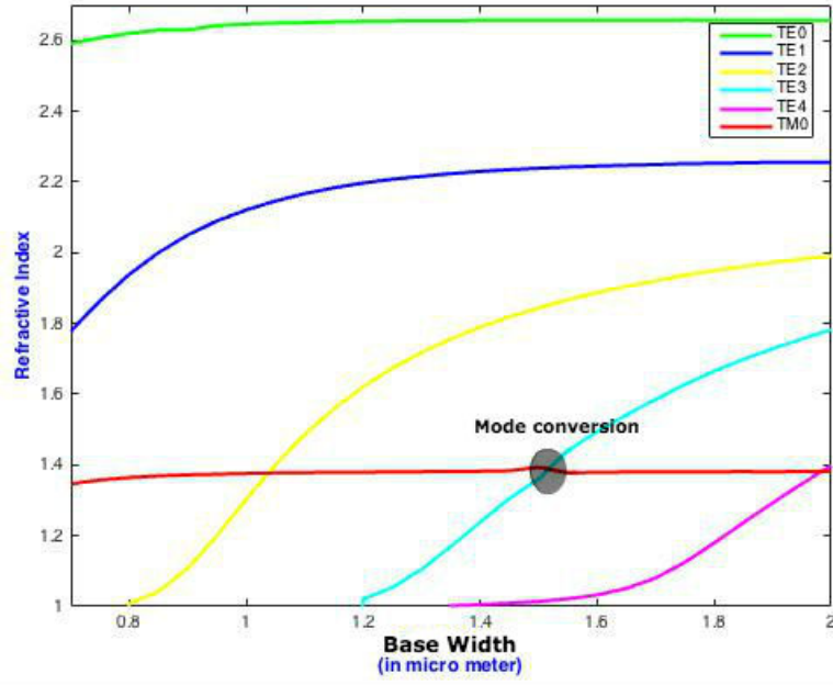
Figure 4.20: TE and TM modes at different base widths obtained using COMSOL mode solvers
