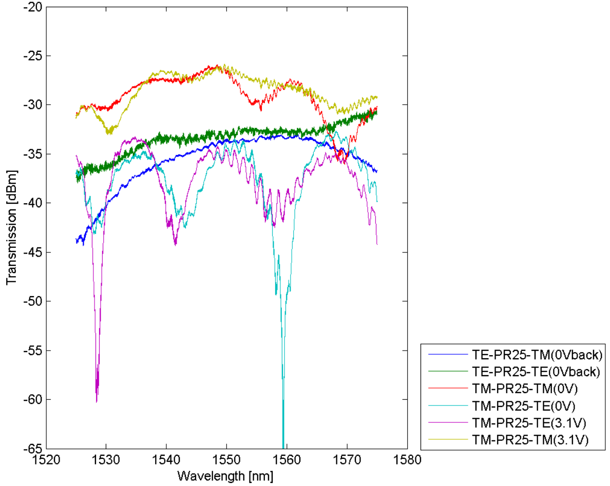
Figure 6.4: TPR with TM input at different voltage inputs for L_\pi = 25 \mu\text{m}
