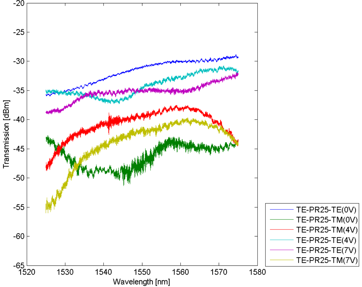
Figure 6.3: TPR with TE input at different voltage inputs for L_\pi = 25 \mu\text{m}
