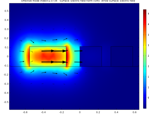
Figure 4.24: No TE coupling in PBS slot waveguide at the mode coupling region
