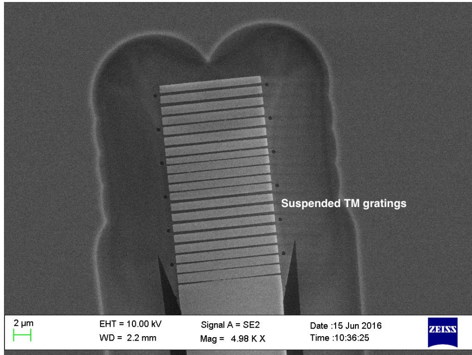
Figure 5.7: TM suspended gratings viewed under SEM
