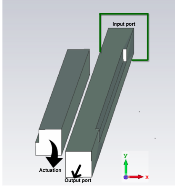
Figure 4.12: Design of single-stair waveguide with MEMS tuning waveguide. Stair cross-section dimensions are: \text{Rib}_{\text{width}} = 200 \text{ nm} , \text{Rib}_{\text{height}} = 110 \text{ nm} , \text{Slab}_{\text{width}} = 230 \text{ nm} , \text{Slab}_{\text{height}} = 110 \text{ nm} , and Stair cross-section length = 62 \mu\text{m} , in both the PR waveguide and MEMS waveguide. The output port is along the Z-axis
