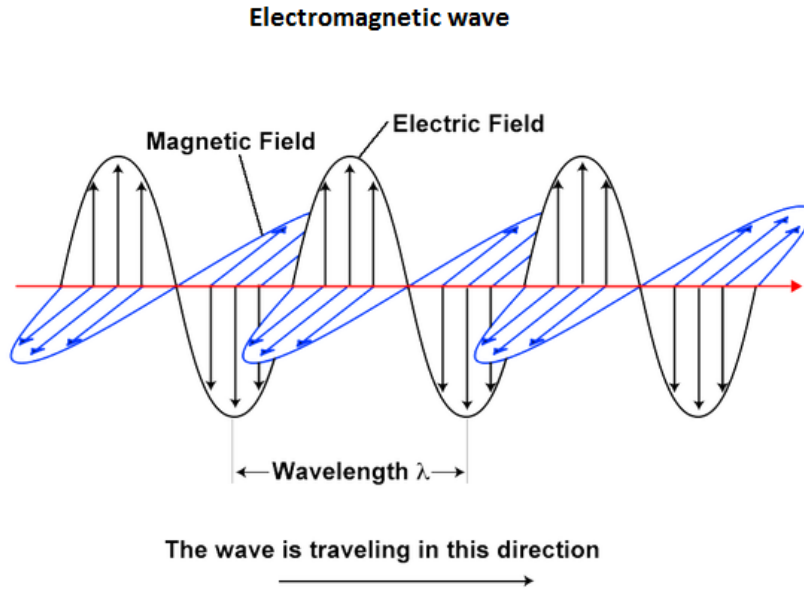
Figure 2.2: Propagation of TEM wave
