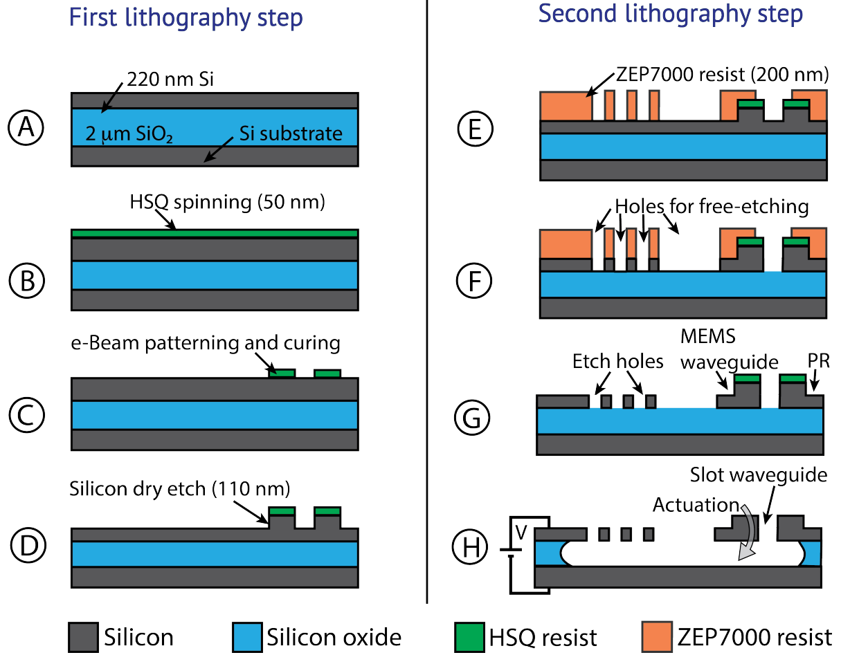
Figure 5.1: A cross-sectional schematic of the fabrication process
