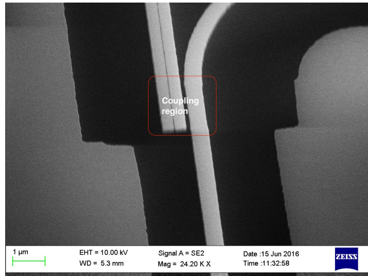
Figure 5.2: Suspended PBS with TM cross-port and TE through
