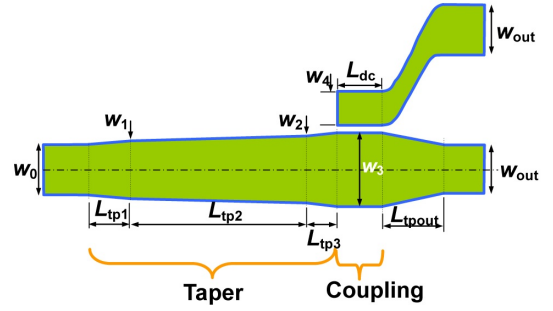
(b) Schematic of the PR
