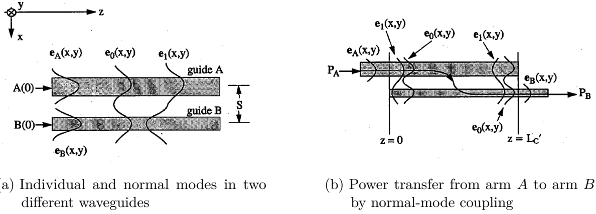
Figure 2.8: Description of the directional coupler under coupled-mode and normal-mode
