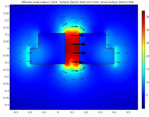
(a) TE mode with the MEMS cross-section
