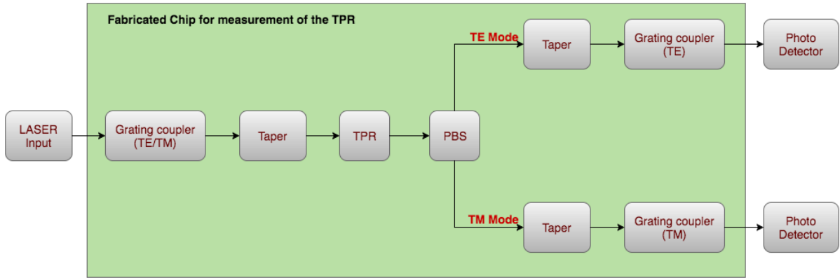
Figure 4.17: System level block diagram of the fabricated measurement setup
