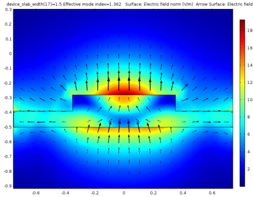
(a) TE mode with Base width = 1500 nm
