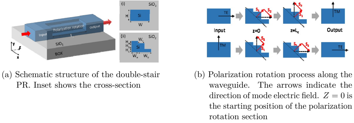
Figure 3.5: PR using double-stair waveguide mode hybridization, by Xie et al. [30]
