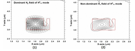
(b) Contour plots of (1) the dominant H_y field profile and (2) the non-dominant H_x field profile of the H_{11}^y mode with W = 800\text{nm} and H = 800\text{nm} , t_w = 100\text{nm} and t_h = 400\text{nm}
