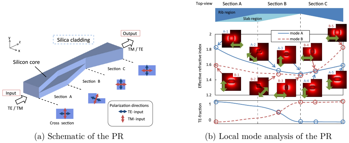
Figure 3.3: PR using mode evolution, by Goi et al. [54]
