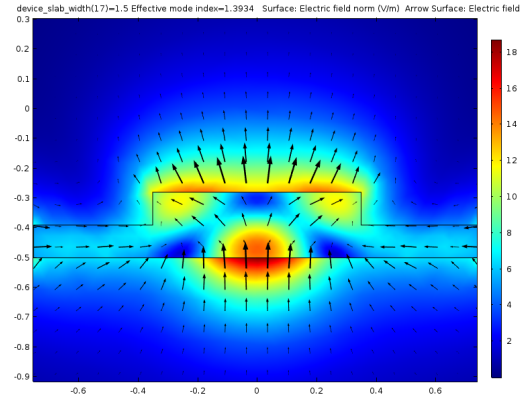
(b) TM mode with Base width = 1500 nm
