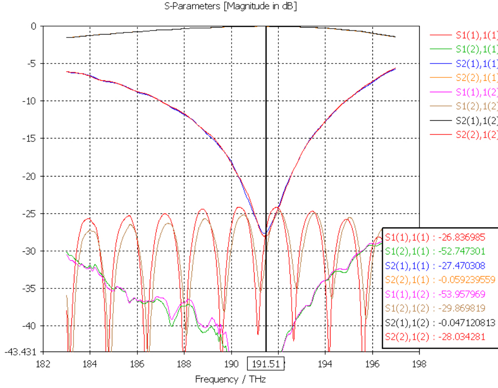
Figure 4.7: Simulated S-parameters in the single-stair waveguide with initial dimensions at the port as width = 230 nm and height = 220 nm. Stair cross-section dimensions are: Rib width = 200 nm, Rib height = 110 nm, Base width = 230 nm, Slab height = 110 nm, and cross-section length = 62 \mu\text{m} obtained using CST 3-D simulation
