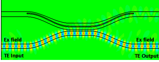
(a) TE mode through
