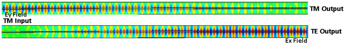
Figure 4.9: TM-TE mode conversion along the waveguide with decreasing E_y field and increasing E_x field
