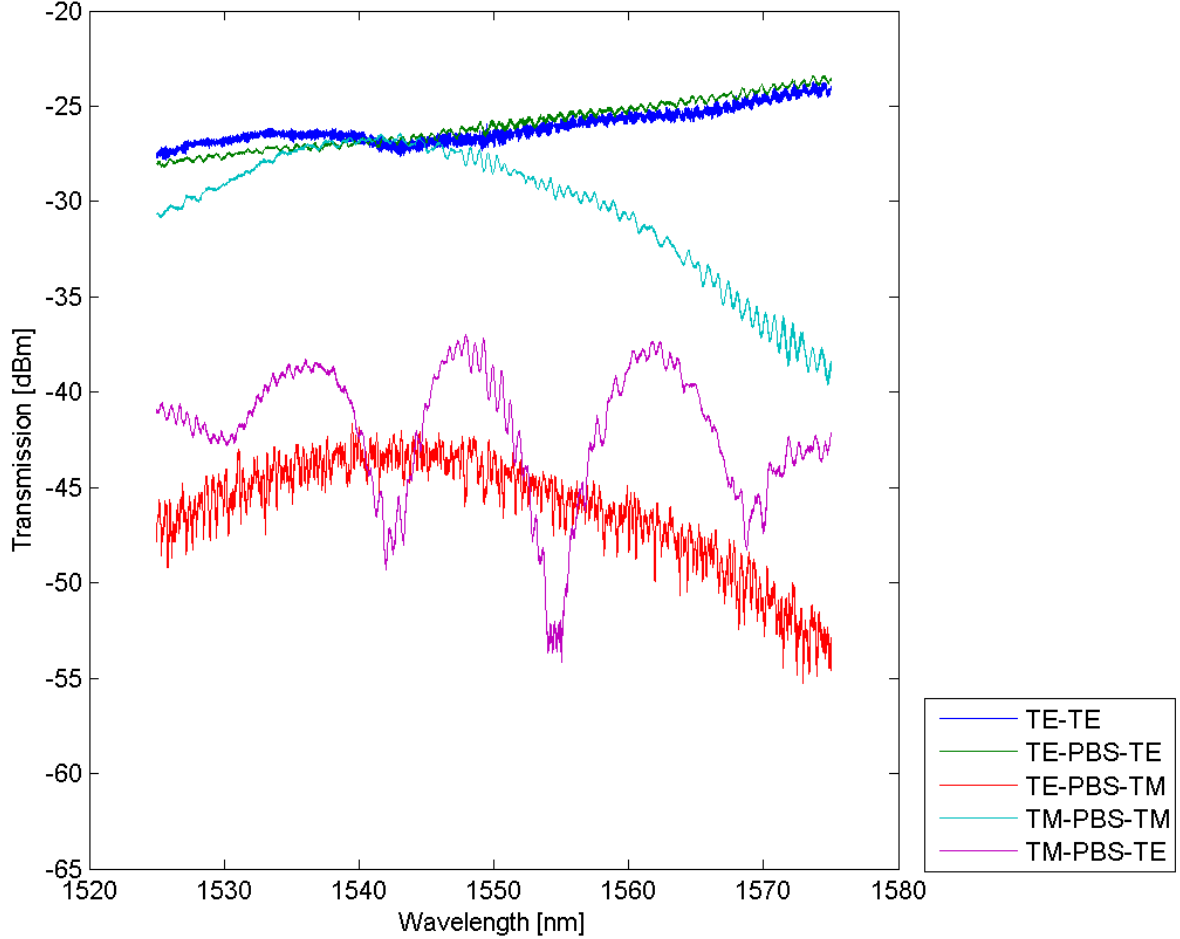
Figure 6.1: PBS with TE/TM input
