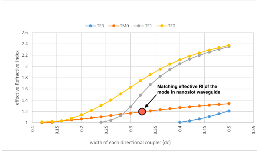
Figure 4.23: Effective RI for different dimensions of slot cross-section
