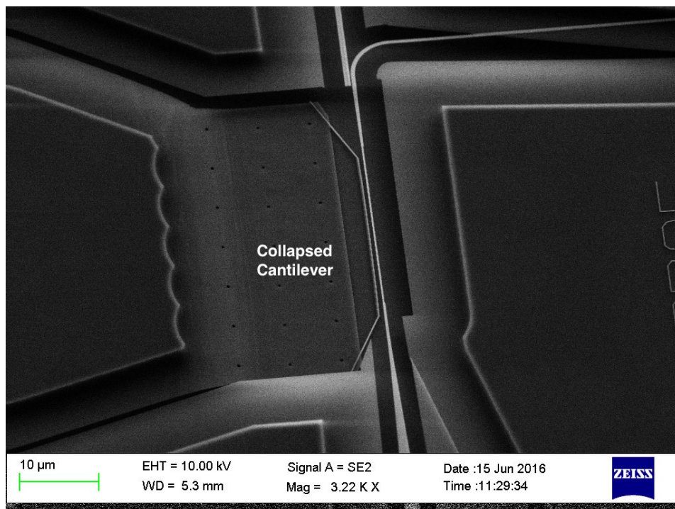
Figure 5.8: Stiction problem on applying a voltage more than the pull in voltage
