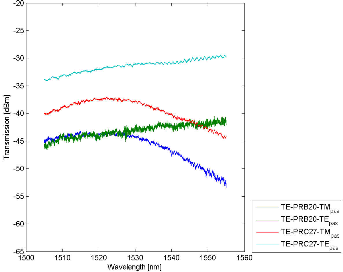
Figure 6.2: Passive PR with TE input for different cross-section lengths
