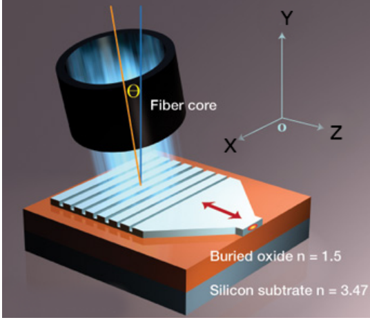
(a) Fiber to waveguide surface coupling using grating coupler
