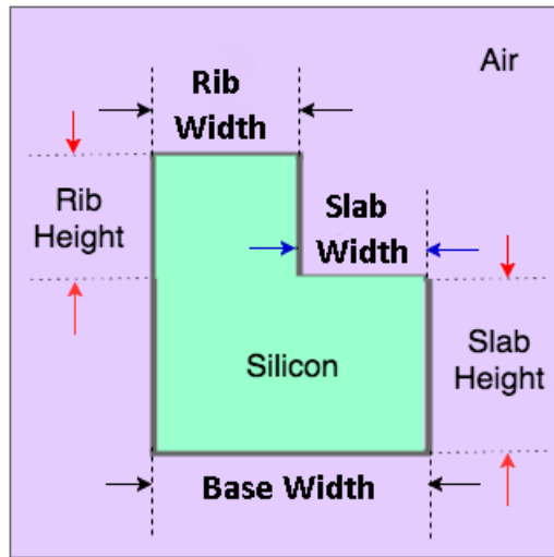
Figure 4.1: Stair waveguide geometry
