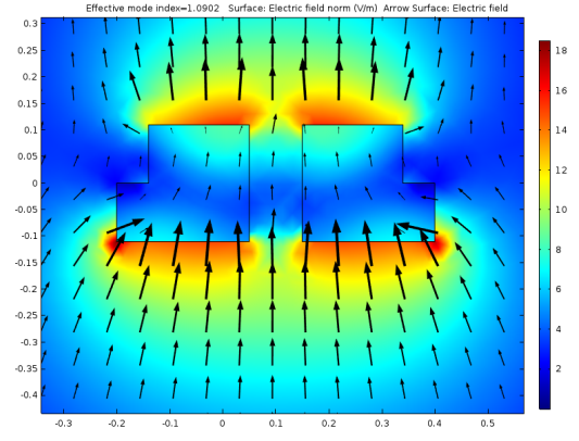
(b) TM mode with the MEMS cross-section
