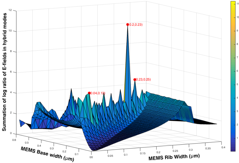
Figure 4.10: Summation of real part of absolute value of the logarithmic ratio of E_x and E_y fields plotted against rib and total width in an area chart using MATLAB
