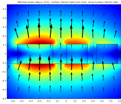
(a) Phase matched TM coupling in the mode coupling cross-section
