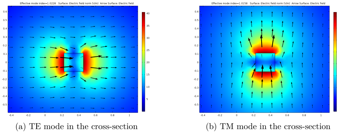
Figure 4.4: Fundamental modes in the cross-section with \text{Width} = 230 \text{ nm} , \text{Height} = 220 \text{ nm} , obtained using Comsol 2-D eigenmode simulation
