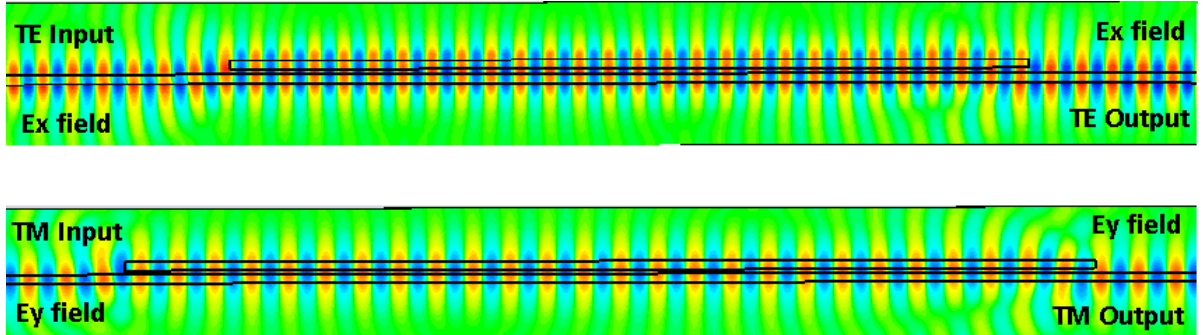
Figure 4.13: TPR transmission in silica cladding without MEMS waveguide actuation
