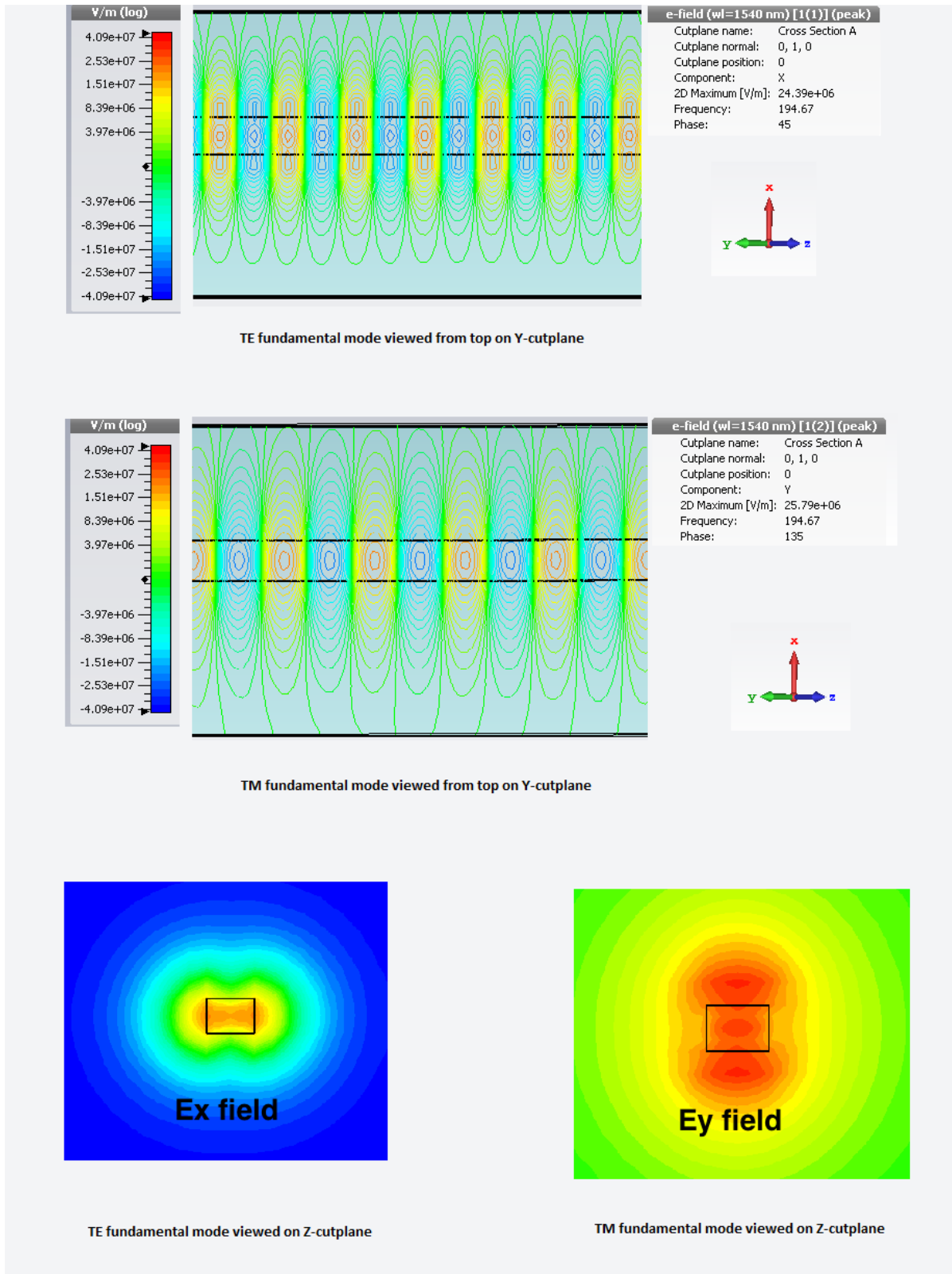
Figure 2.4: Transverse Electric (TE) and Transverse Magnetic (TM) fundamental mode in a waveguide using CST simulation
