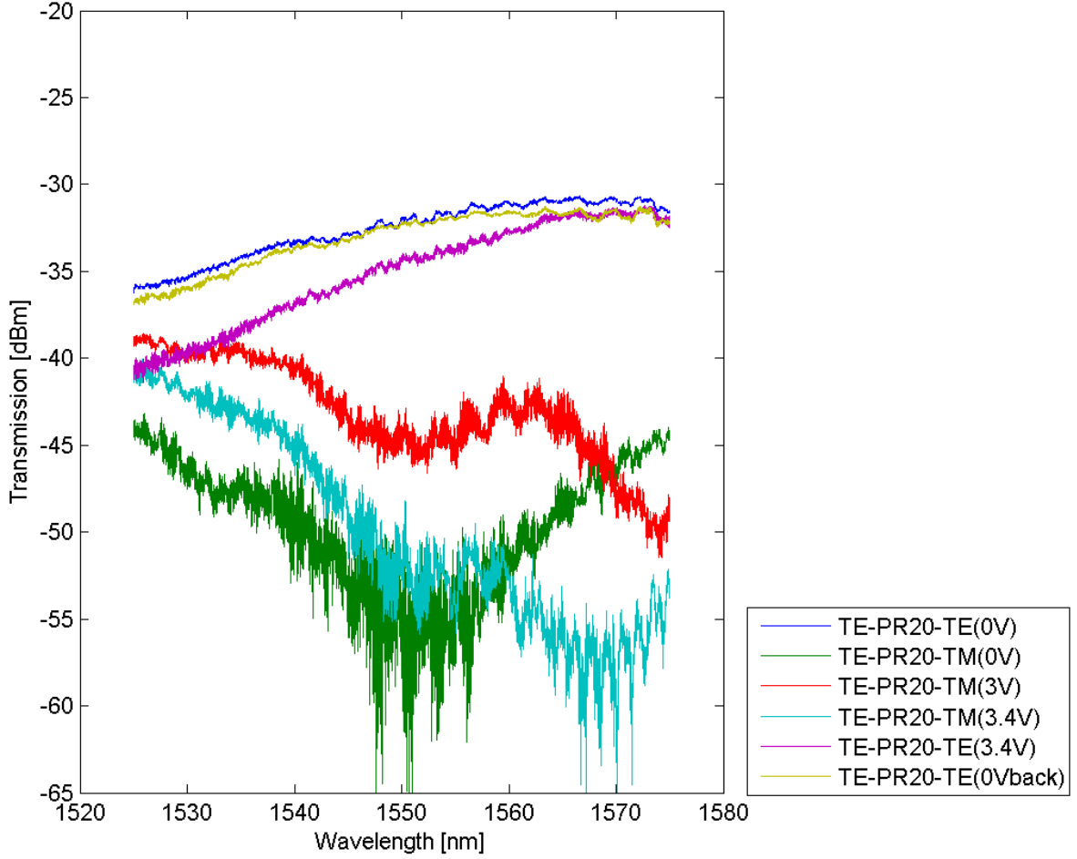
Figure 6.5: TPR with TM input at different voltage inputs for L_\pi = 20 \mu\text{m}
