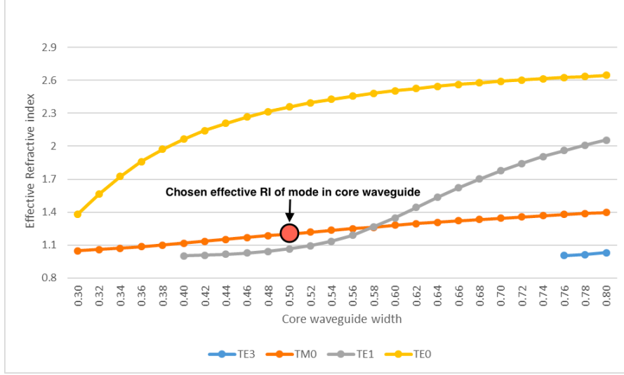
Figure 4.22: Effective RI for different dimensions of core waveguide width
