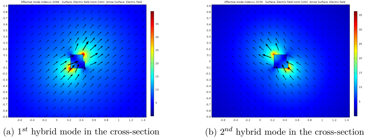
Figure 4.3: Fundamental hybrid modes in the cross-section with \text{Rib}_{\text{width}} = 200 \text{ nm} , \text{Rib}_{\text{height}} = 110 \text{ nm} , \text{Base}_{\text{width}} = 230 \text{ nm} , \text{Slab}_{\text{height}} = 110 \text{ nm} , obtained using Comsol 2-D eigenmode simulation
