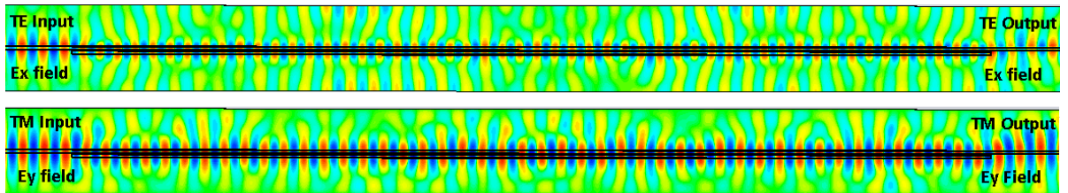
Figure 4.14: TPR transmission in air cladding without MEMS waveguide actuation
